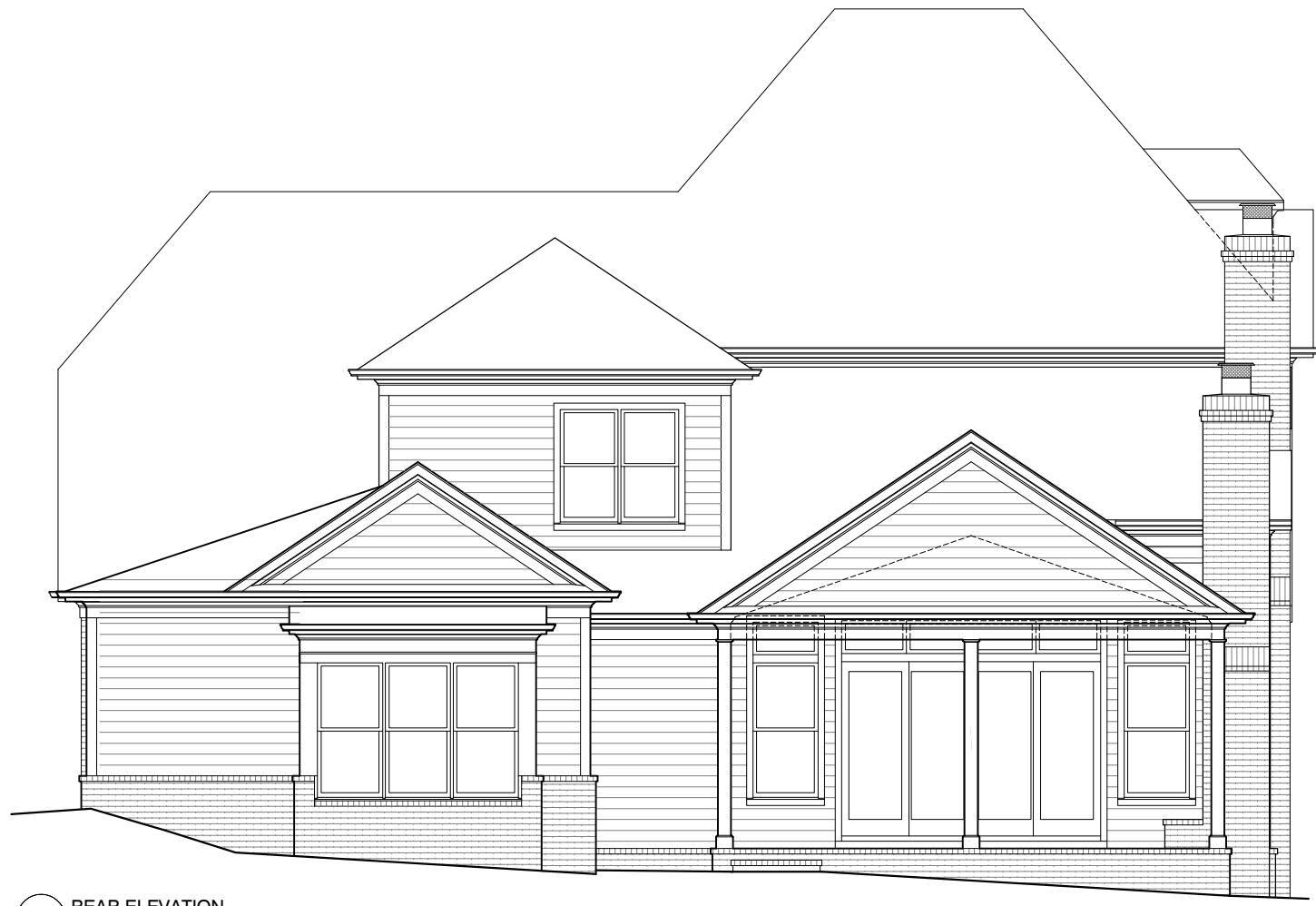
2 REAR ELEVATION 1/8" = 1'-0"
